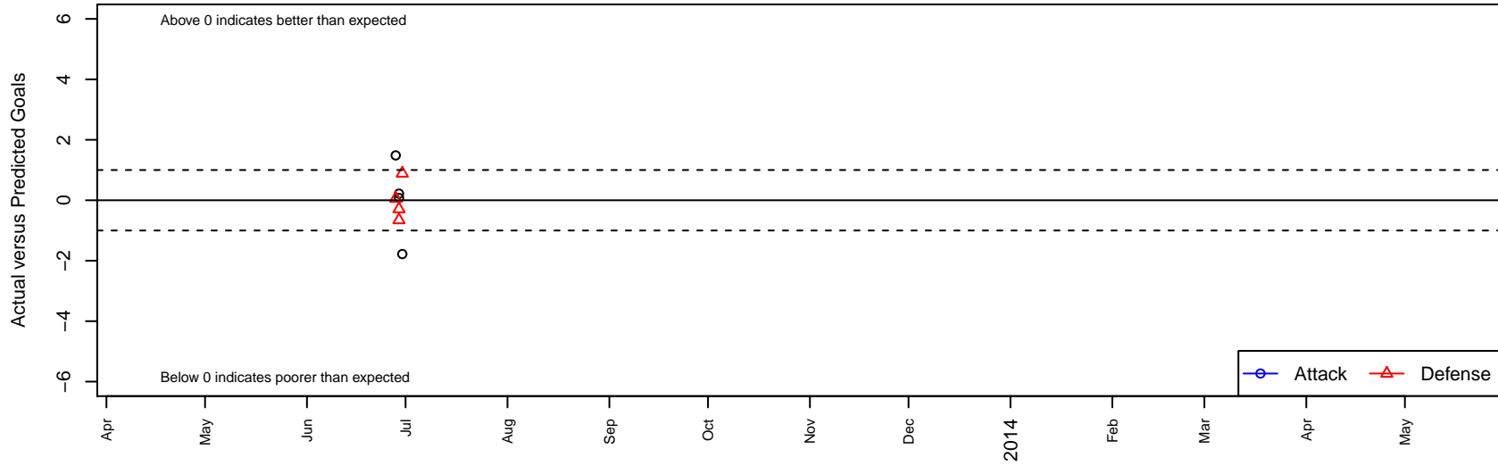
Salem Liverpool B00 Dots are actual minus expected GF (blue circles) and GA (red triangles). Blue line is smoothed change in attack strength. Red is smoothed change in defense strength.
